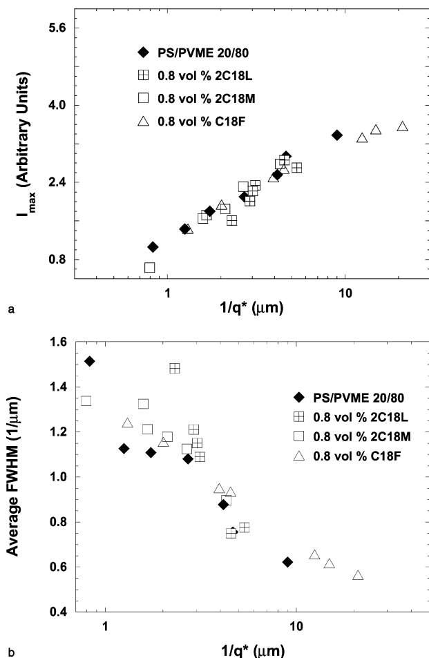
Figure 11. Maximum intensities (a) and the averages of the left and right fwhm (b) of the peak in the Fourier power spectra graphed against 1/q^* for the unfilled \phi_{\text{PS}} = 0.18 blend and the nanocomposites with 0.8 vol % 2C18L, 2C18M, and C18F. A lower 1/q^* value corresponds to a smaller length scale and therefore a less developed phase-separated morphology.
