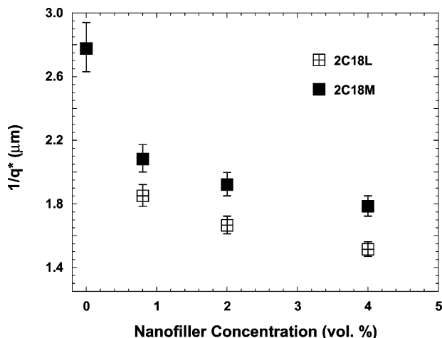
Figure 10. Characteristic length scale ( 1/q^* ) of the phase-separated structure in a blend film with \phi_{\text{dPS}} = 0.28 as a function of 2C18L and 2C18M concentration, obtained from FFT of AFM images. The effect of the layered silicate on the phase-separated morphology increases with the concentration. For a given concentration, the 2C18L has a larger effect than the 2C18M.
