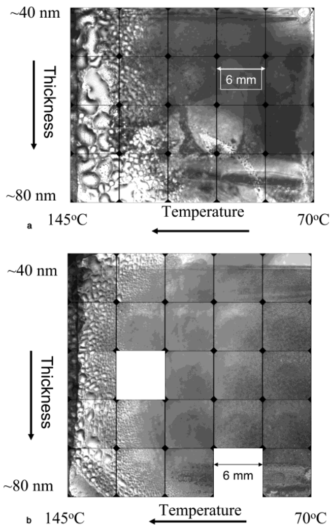
Figure 15. 2.5 \times magnified optical microscopy images of the low molecular weight PS ( M_w = 3680 ) with no layered silicate (a) and 0.8 vol % 2C18M (b) on hydrophobic Si wafers. As expected, film disruption occurs most strongly at higher temperatures and larger thicknesses. Also, the presence of the layered silicate suppresses the dewetting significantly.
