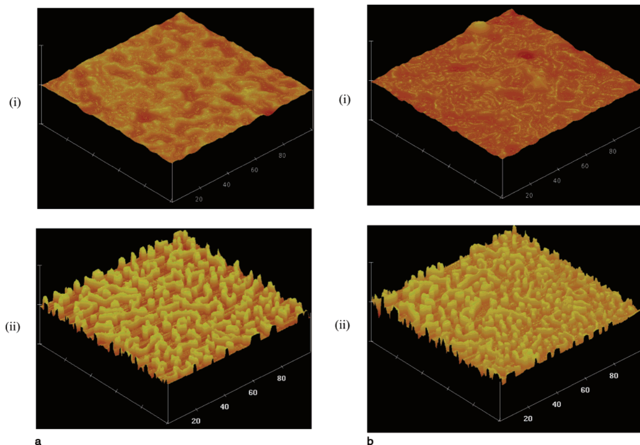
Figure 3. 3D topographical AFM images showing the phase-separated morphology in the \phi_{PS} = 0.18 blend film at T^\circ = -13^\circ\text{C} (a) and the \phi_{PS} = 0.18 blend film with 0.8 vol % 2C18M at T^\circ = -9^\circ\text{C} (b). Part i corresponds to annealed films, while part ii refers to images taken after the methanol wash. The height scale in all images is 3\text{ }\mu\text{m} , and the lateral dimensions are 100\text{ }\mu\text{m} \times 100\text{ }\mu\text{m} . Note that the phase-separated morphology is clearly visible for the unfilled blend in both cases, although the methanol wash significantly increases the contrast. For the 2C18M-containing blend, on the other hand, the phase-separated morphology is not very well-defined before the methanol wash. This lack of definition compared to the unfilled blend is representative of all images of layered-silicate-containing images.
