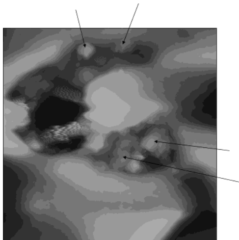
Figure 14. 5.7\ \mu\text{m} \times 5.7\ \mu\text{m} AFM image showing the phase-separated morphology after 15 min of annealing at 177\ ^\circ\text{C} for the nanocomposite with \phi_{\text{DPS}} = 0.28 and containing 2.0 vol % 2C18L. Note that the layered-silicate particles (marked by arrows) seem to favor the PVME-rich phase.
